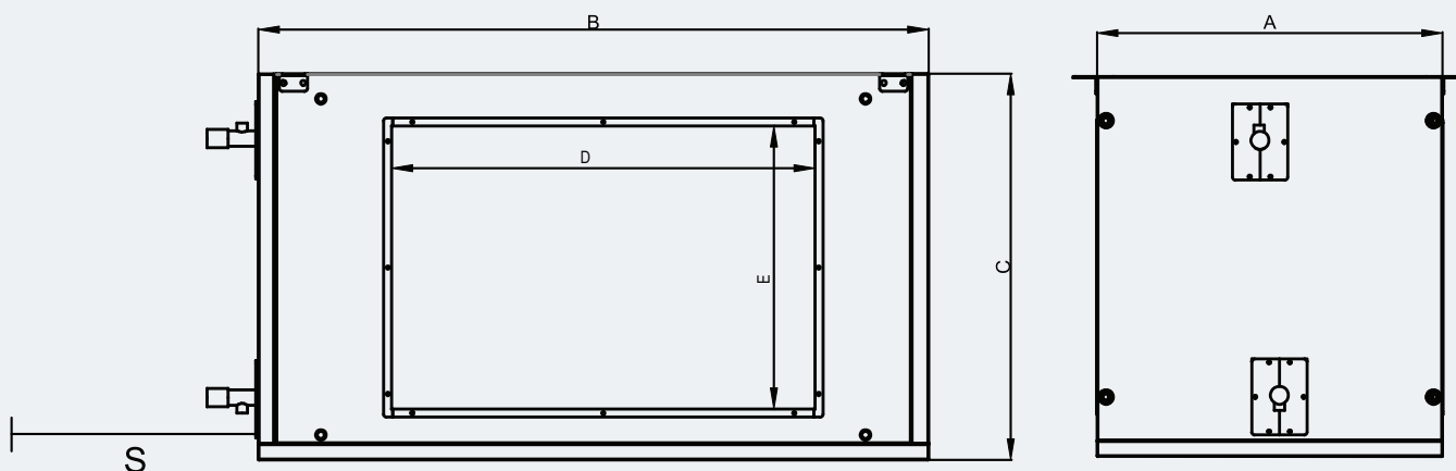
Cooling Coil
