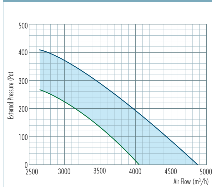
Performance Curve
