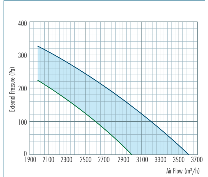
Performance Curve
