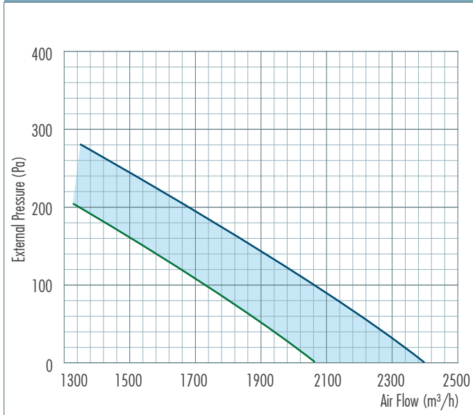
Performance Curve
