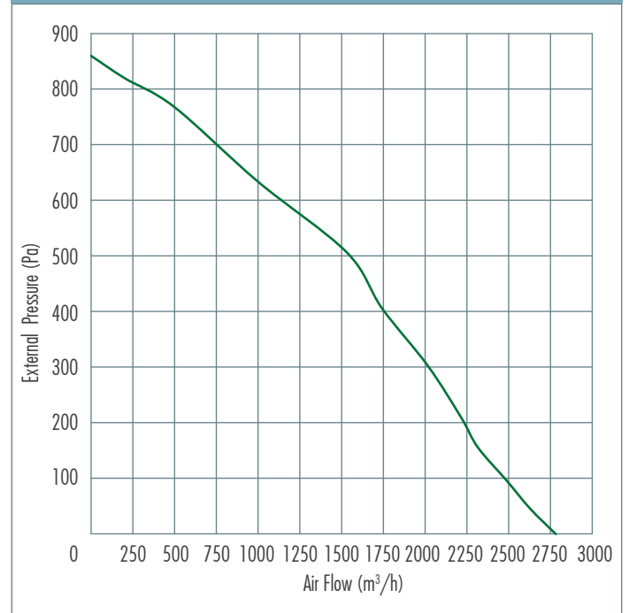
Performance Curve
