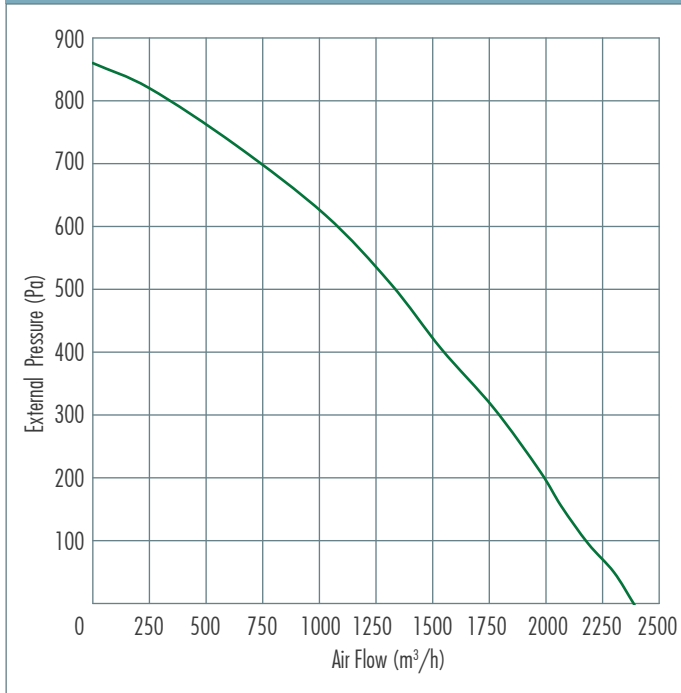
Performance Curve
